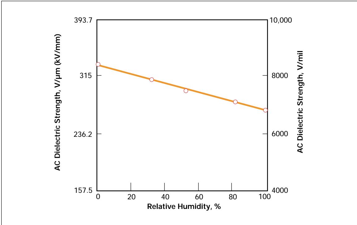
Figure 11. AC Dielectric Strength vs. Relative Humidity, Type HN Film, 25 μm (1 mil)
