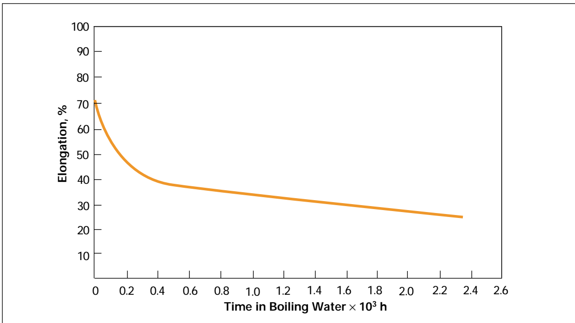
Figure 4. Ultimate Elongation After Exposure to 100°C (212°F) Water, Type HN Film, 25 μm (1 mil)
